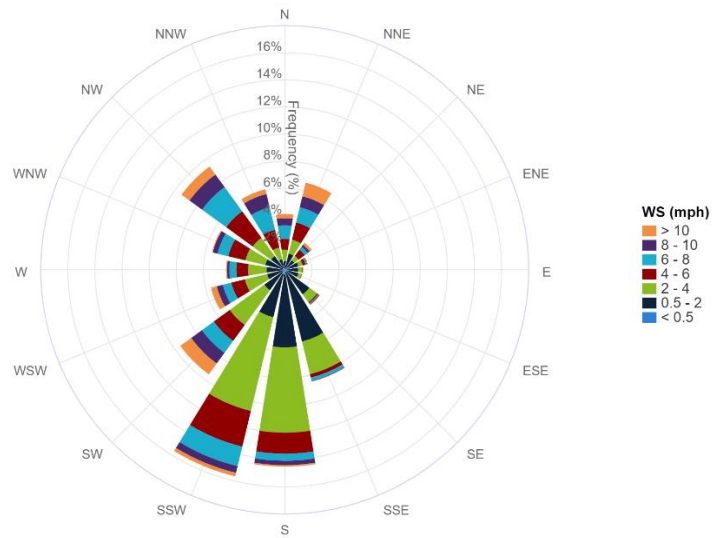
7-Day Wind Rose Plot [From 05/24/2024 00:00 to 05/30/2024 23:59]
